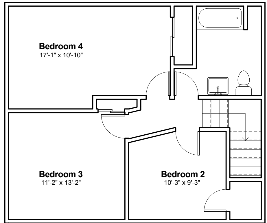
2nd Floor
